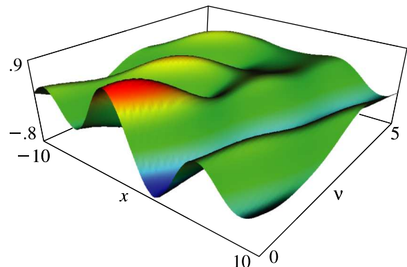
Figure 11.10.4: Weber function E_\nu(x) for -10 \leq x \leq 10 and 0 \leq \nu \leq 5 .
