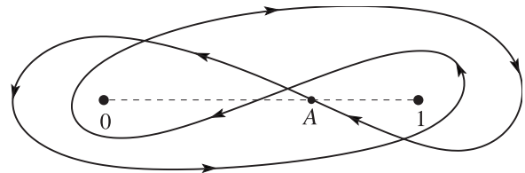
Figure 15.6.1: t -plane. Contour of integration in (15.6.5).
