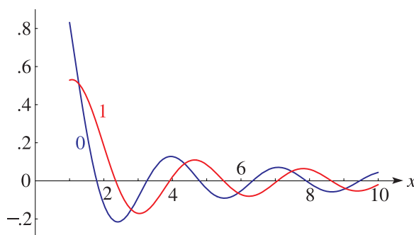
Figure 30.11.1: S_n^{0(1)}(x, 2) , n = 0, 1 , 1 \leq x \leq 10 .
