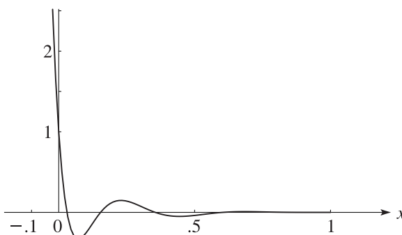
Figure 15.3.2: F(5, -10; 1; x) , -0.023 \leq x \leq 1 .
