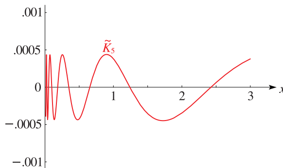
Figure 10.26.10: \tilde{K}_5(x), 0.01 \leq x \leq 3 .
