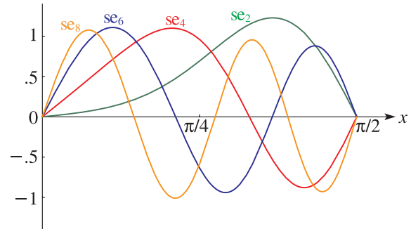
Figure 28.3.8: se_{2n}(x, 10) for 0 \leq x \leq \pi/2 , n = 1, 2, 3, 4 .
