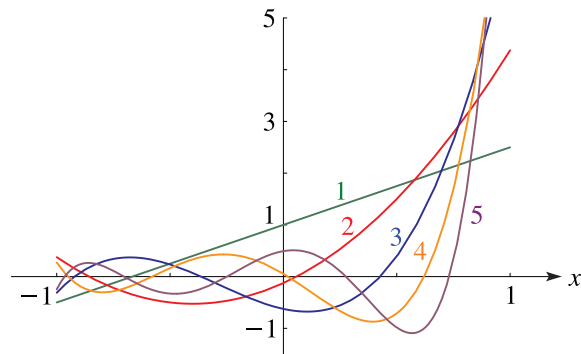
Figure 18.4.1: Jacobi polynomials P_n^{(1.5,-0.5)}(x) , n = 1, 2, 3, 4, 5 .
