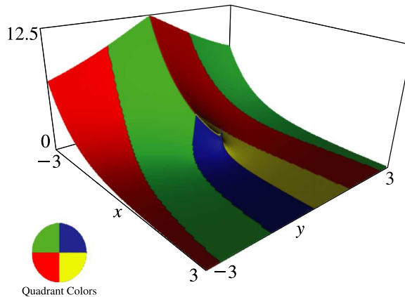
Figure 8.3.8: \Gamma(0.25, x + iy) , -3 \leq x \leq 3 , -3 \leq y \leq 3 . Principal value. There is a cut along the negative real axis. When x = y = 0 , \Gamma(0.25, 0) = \Gamma(0.25) = 3.625 \dots
