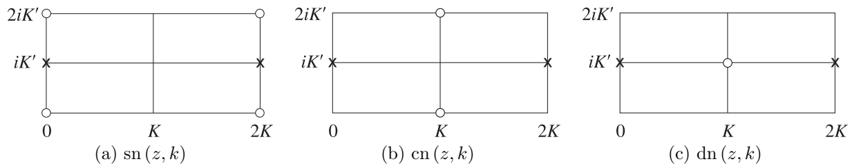
Figure 22.4.1: z -plane. Poles \times \times \times and zeros \circ \circ \circ of the principal Jacobian elliptic functions.
