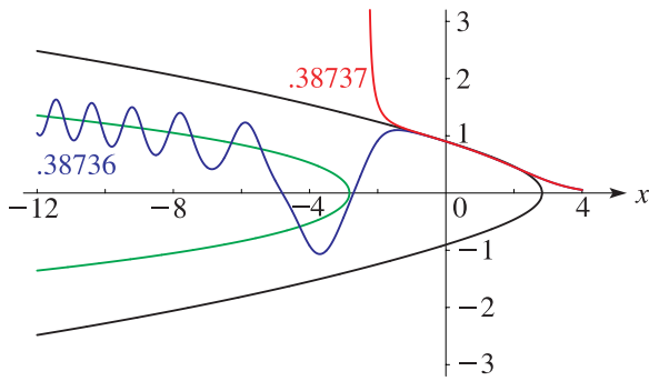
Figure 32.3.9: u_k(x; \frac{5}{2}) for -12 \leq x \leq 4 with k = 0.38736, 0.38737 . The two graphs are indistinguishable when x exceeds -1.0 , approximately. The curves u^2 + \frac{1}{3}x \pm \frac{1}{6}\sqrt{x^2 + 24} = 0 are shown in green and black, respectively.
