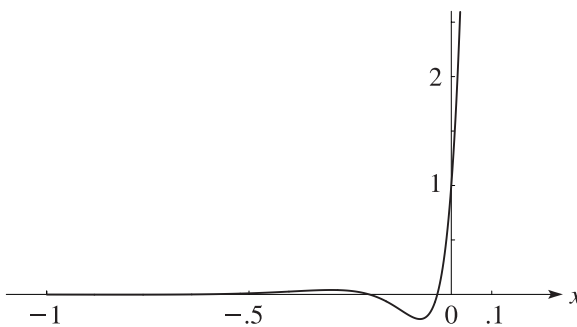
Figure 15.3.4: F(5, 10; 1; x) , -1 \leq x \leq 0.022 .
